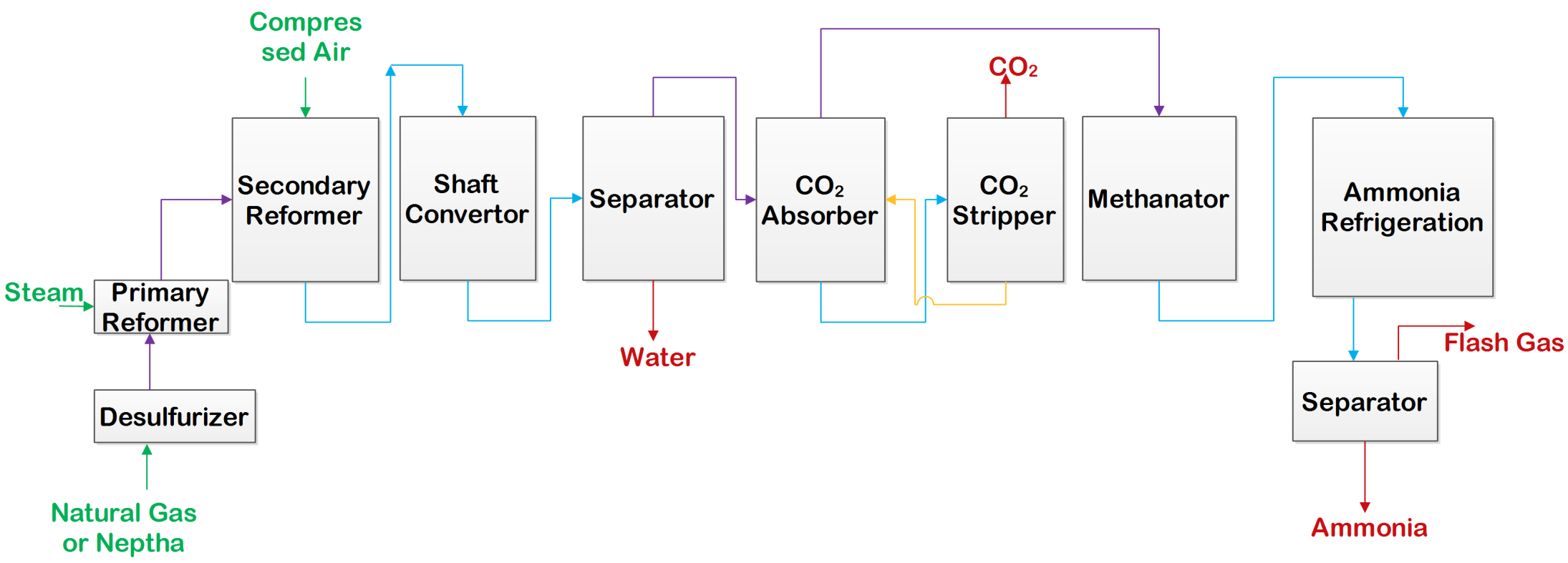
Figure: Manufacturing of Ammonia By Kellogg Process
